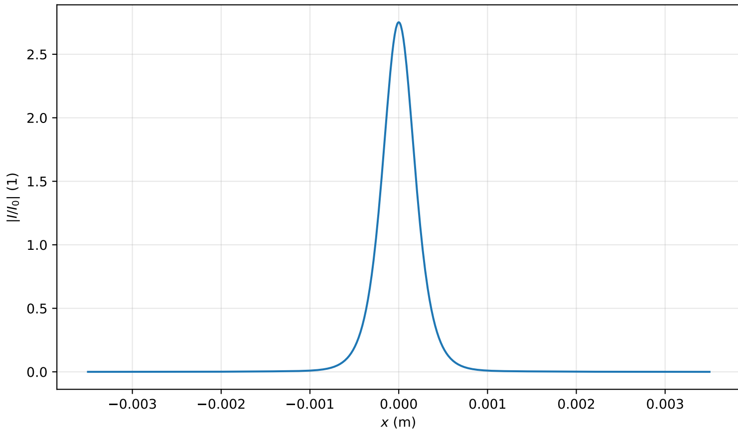
Intensity profile I(x, y = 0, z = 3.184m)/I_0 , P_{in}=1.0P_{cr} , artificial time
